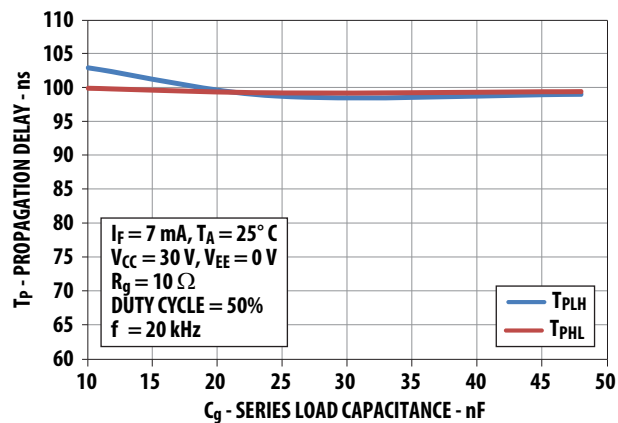
Figure 18 Propagation Delay vs. C_g
