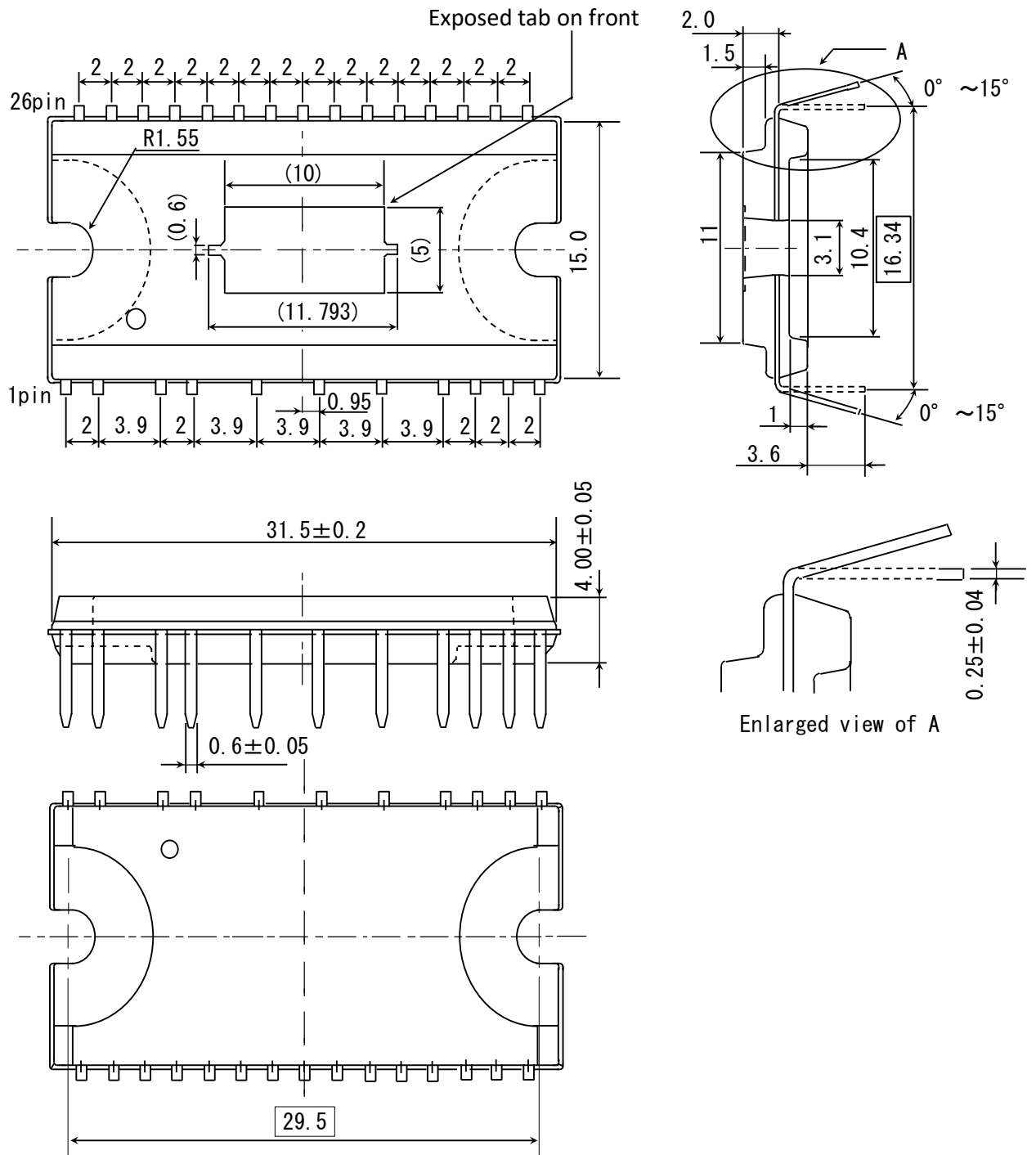
FIGURE C: Dimensions of DIP26N
