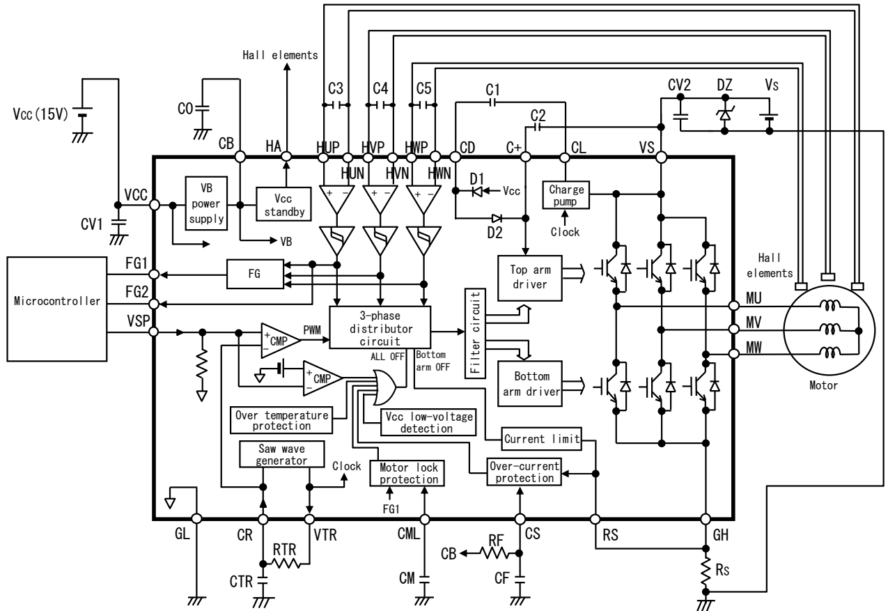
FIGURE 1.3.1 Block Diagram
