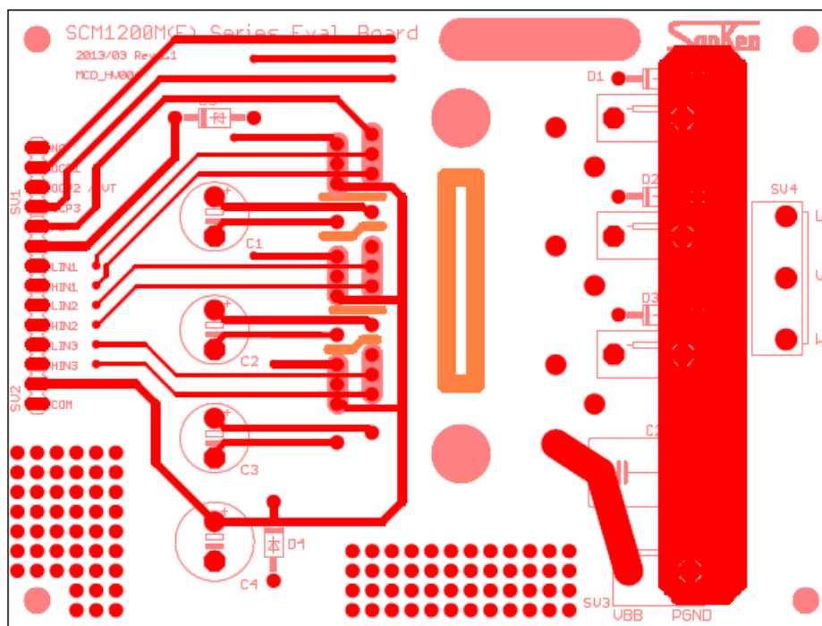
Figure 16-1. Top view
