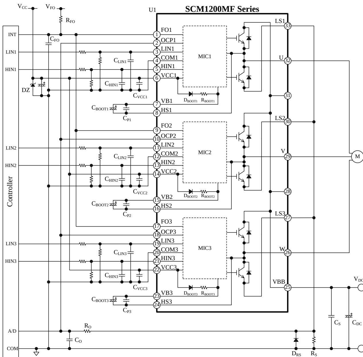
Figure 9-2. Typical application using shingle shunt resistor
