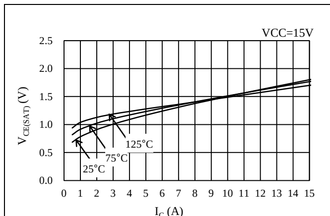
Figure 15-29. IGBT V_{CE(SAT)} vs. I_C
