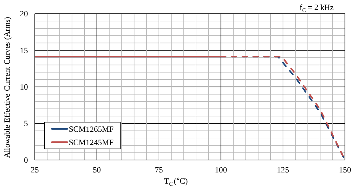
Figure 15-71. Allowable effective current, 20 A device ( f_C = 2 kHz)
