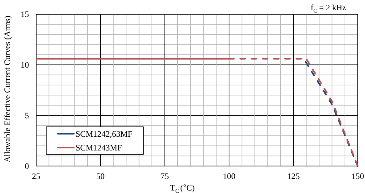
Figure 15-69. Allowable effective current, 15 A device ( f_C = 2 kHz)
