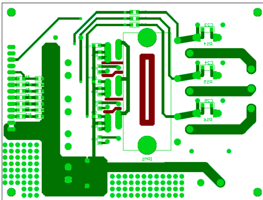
Figure 16-2. Bottom view
