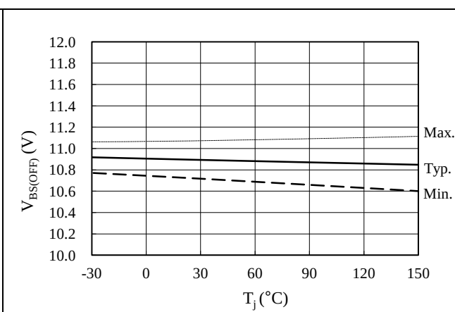
Figure 15-18. Logic Operation Stop Voltage, V_{BS(OFF)} vs. T_j
