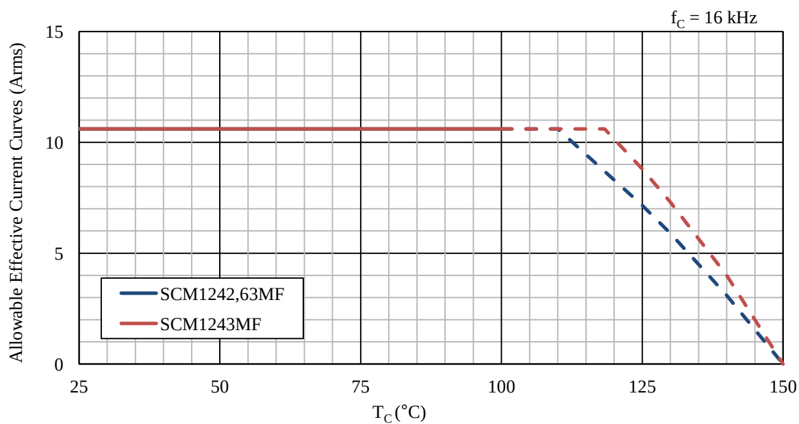
Figure 15-70. Allowable effective current, 15 A device ( f_C = 16 kHz)
