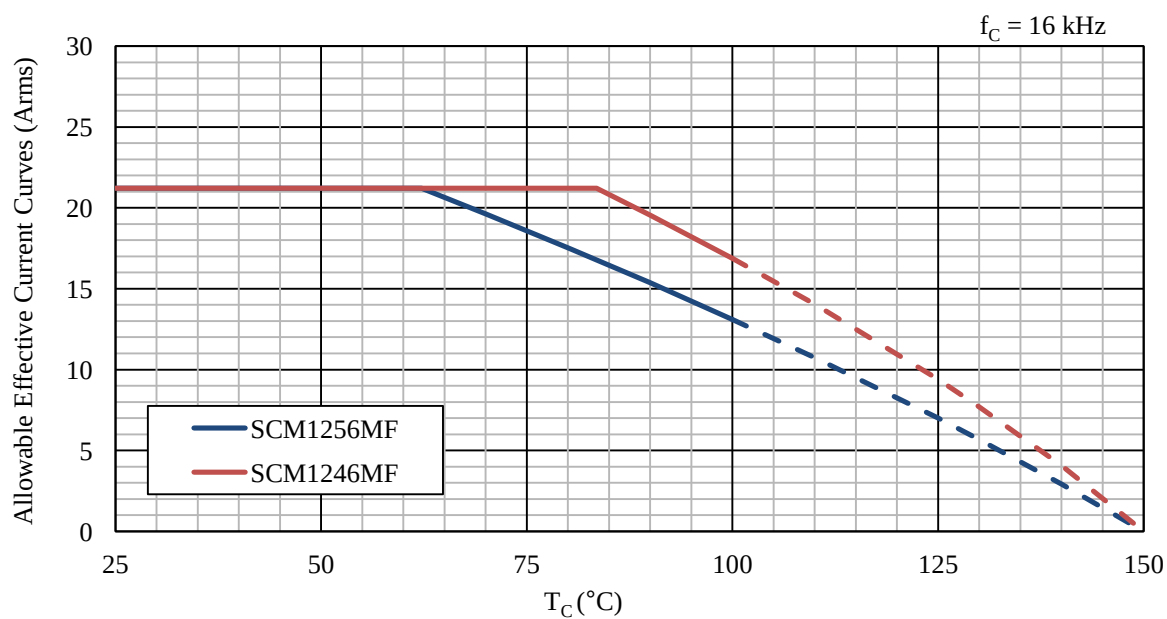
Figure 15-74. Allowable effective current, 30 A device ( f_C = 16 kHz)
