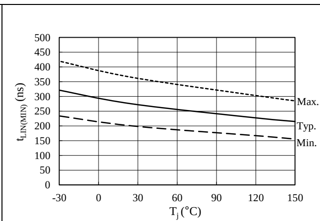
Figure 15-14. Minimum transmittable pulse width for low-side switching, t_{LIN(MIN)} vs. T_j
