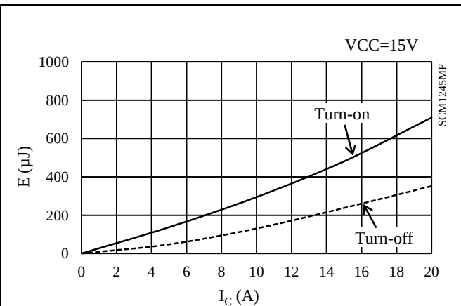
Figure 15-56 Low-side switching loss ( T_j = 25^\circ\text{C} )
