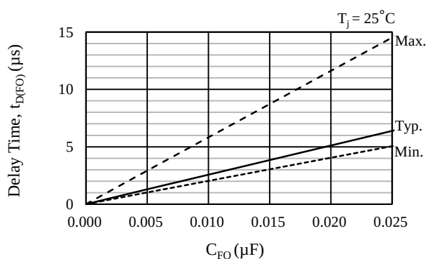
Figure 12-11. Delay time, t_{D(FO)} vs. filter capacitor, C_{FO}
