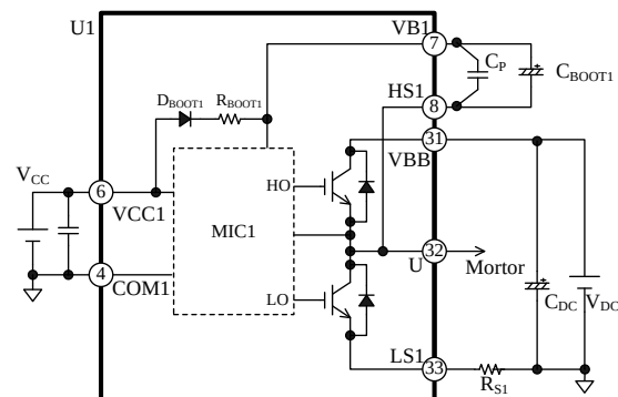
Figure 12-1. Bootstrap circuit
