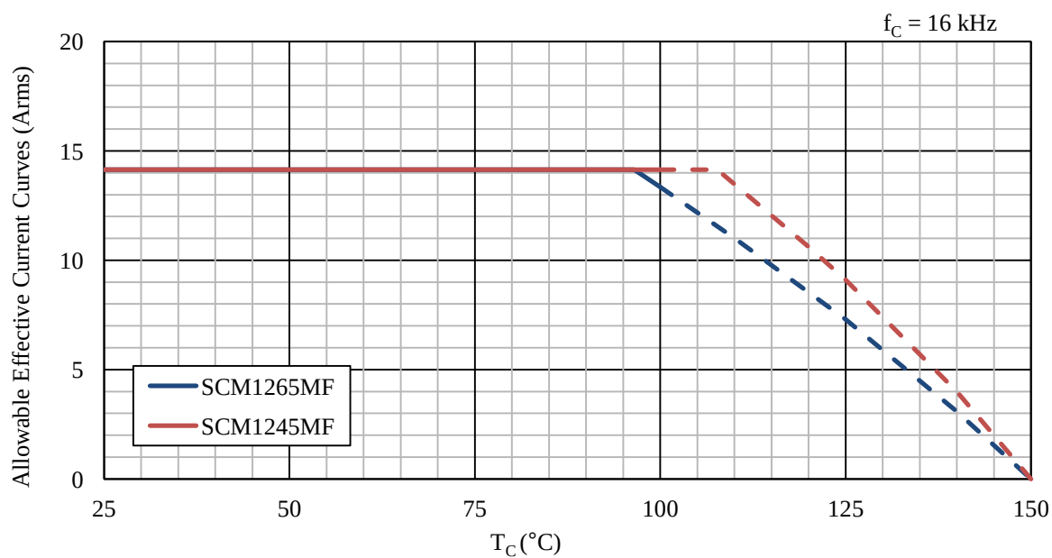
Figure 15-72. Allowable effective current, 20 A device ( f_C = 16 kHz)
