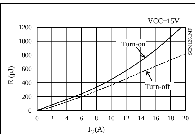
Figure 15-38. Low-side switching loss ( T_j = 125^\circ\text{C} )
