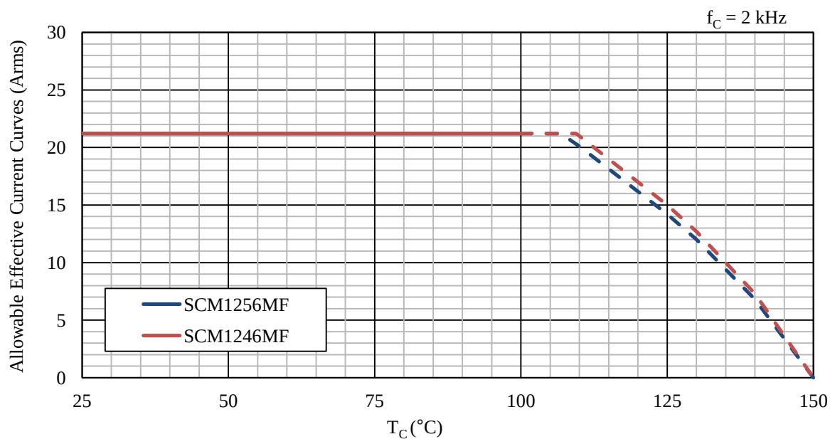
Figure 15-73. Allowable effective current, 30 A device ( f_C = 2 kHz)
