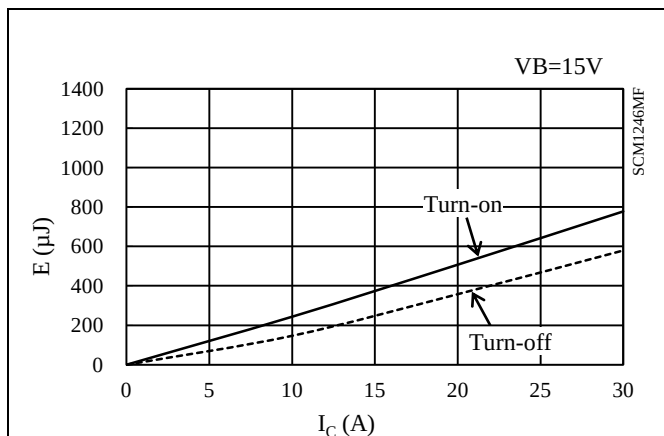
Figure 15-63 High-side switching loss ( T_j = 25^\circ\text{C} )
