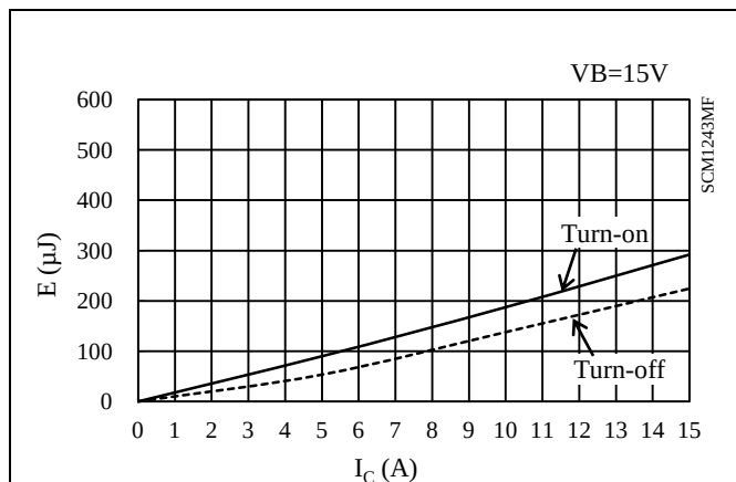
Figure 15-47 High-side switching loss ( T_j = 25^\circ\text{C} )
