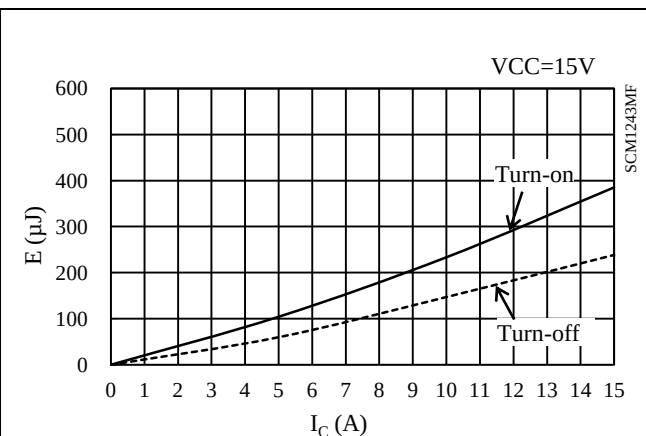
Figure 15-48 Low-side switching loss ( T_j = 25^\circ\text{C} )
