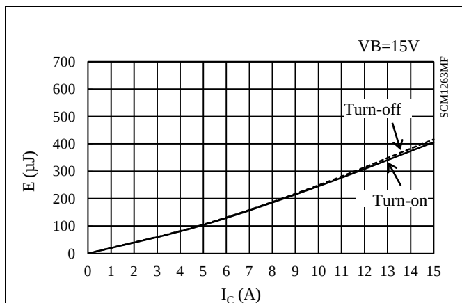
Figure 15-43 High-side switching loss ( T_j = 25^\circ\text{C} )
