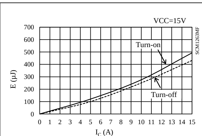
Figure 15-44 Low-side switching loss ( T_j = 25^\circ\text{C} )
