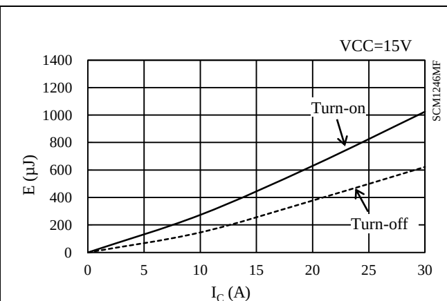
Figure 15-64. Low-side switching loss ( T_j = 25^\circ\text{C} )
