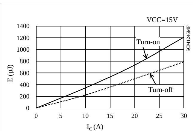
Figure 15-66. Low-side switching loss ( T_j = 125^\circ\text{C} )
