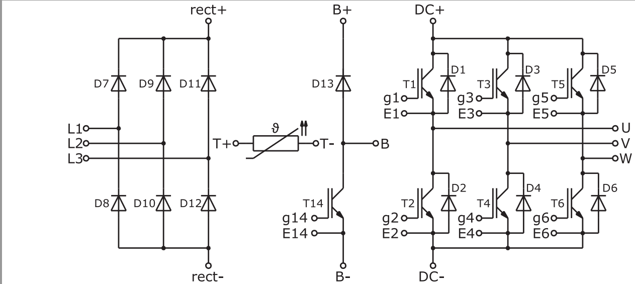
Pinout
