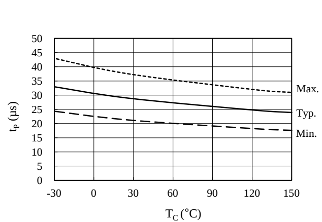
Figure 15-20. OCP Hold Time, t_p vs. T_C
