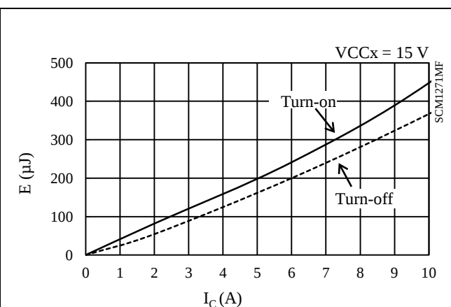
Figure 15-35. Low-side Switching Loss ( T_j = 125\text{ °C} )
