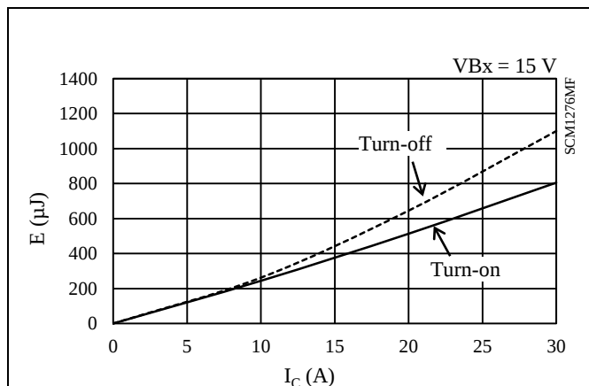
Figure 15-44. High-side Switching Loss ( T_j = 25\text{ }^{\circ}\text{C} )
