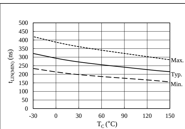
Figure 15-16. Minimum Transmittable Pulse Width for Low-side Switching, t_{LIN(MIN)} vs. T_C
