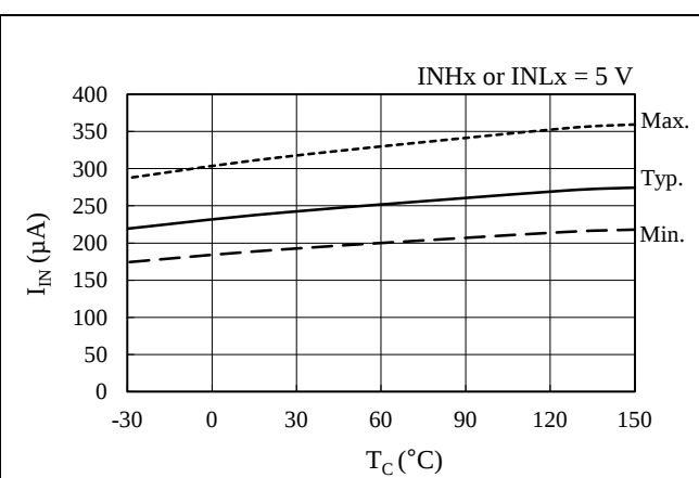
Figure 15-12. Input Current at High Level ( I_{INx} or LINx ), I_{IN} vs. T_C
