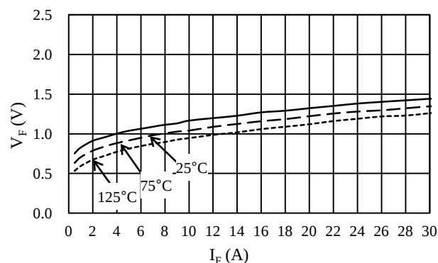
Figure 15-31. Freewheeling Diode V_F vs. I_F
