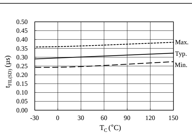
Figure 15-22. SD Pin Filtering Time, t_{FIL(SD)} vs. T_C
