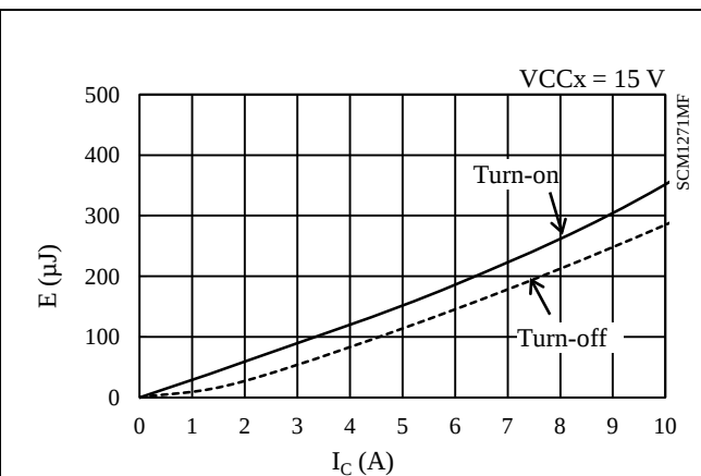
Figure 15-33. Low-side Switching Loss ( T_j = 25\text{ °C} )
